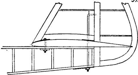
STABILIZER & RUDDER MOUNTING
