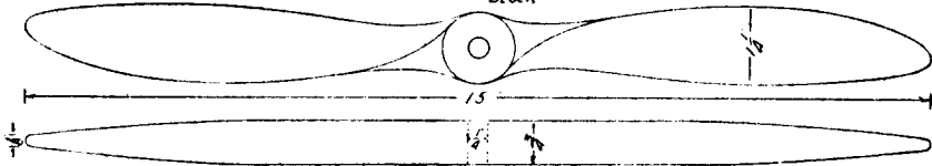
PROP CARVED FROM BASS BLOCK
